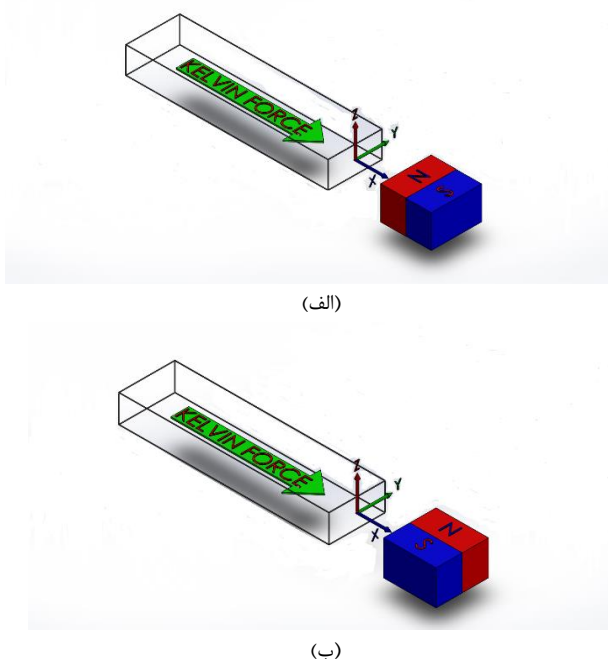
Fig. 1 Schematic picture of FHD Pump-(a) Horizontal magnet with respect to x axis, (b) Vertical magnet with respect to x axis
