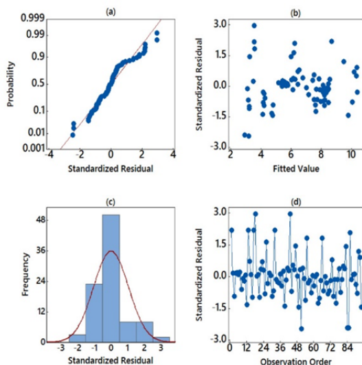
Fig. 3 The results of validation of the MLR regression model
