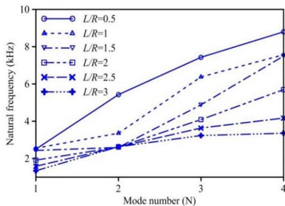
Fig. 13 Natural frequencies of panel with free boundary condition, ( \theta = 3\pi/4 , S=5 )
