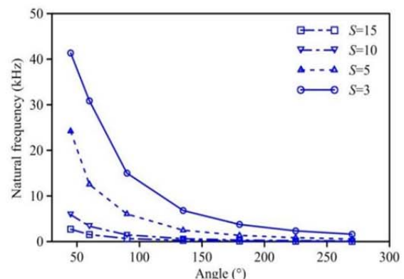
Fig. 12 First natural frequency with free boundary condition ( L=15 mm)
