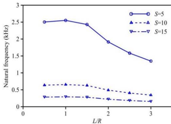
Fig. 14 Effect of radius and length of panel on the first natural frequency ( \theta=3\pi/4 )
