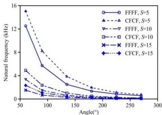
Fig. 15 Effect of boundary condition on the first natural frequency of panel, ( L=15 mm)
