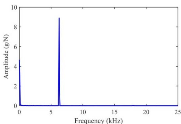
Fig. 11 Frequency response for excitation with hammer
