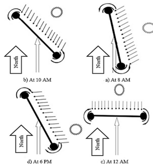
Fig. 3 Working principle of the solar tracker in north-south direction
