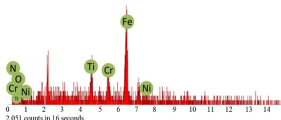
Fig. 14 EDX Of Mix particles with 2 Wt. %
