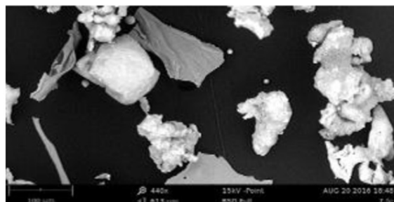
Fig. 1 SEM of stainless steel Powder
