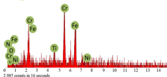
Fig. 15 SEM Of Mix particles with 10 Wt. %
