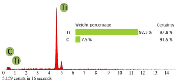
Fig. 5 EDX of TiC Powder
