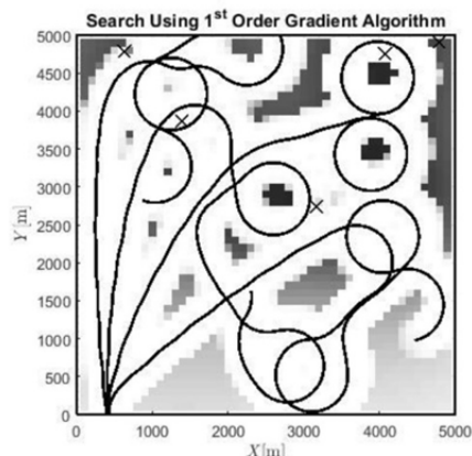
Fig 14 Cooperative Search Using First-Order Gradient Algorithm
