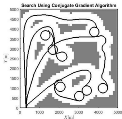
Fig 5 Cooperative Search Using Conjugate Gradient Algorithm
