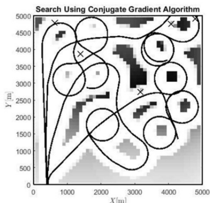
Fig 17 Cooperative Search Using Conjugate Gradient Algorithm
