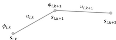
Fig 2 Discrete movement of an agent
