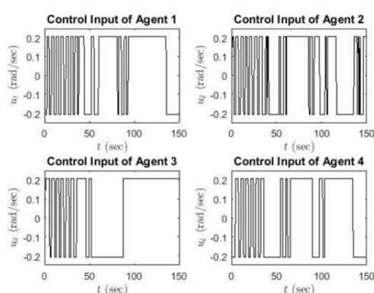
Fig 15 Distributed Control Using First-Order Gradient Algorithm
