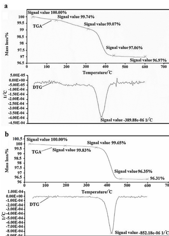
Fig. 10 Mass loss as a result of extended heating (a) PMMA/alumina composite particles (b) PS/alumina composite particles
