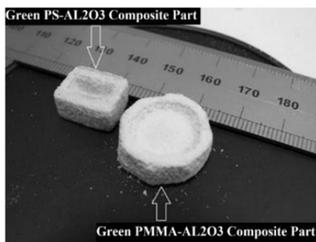
Fig. 12 Complex green parts created with indirect SLS by using one of the best laser parameters (Frequency: 10 kHz, Pulse width: 10 \mu s, laser power: 6 W, scan speed: 100 mm s -1 ).
