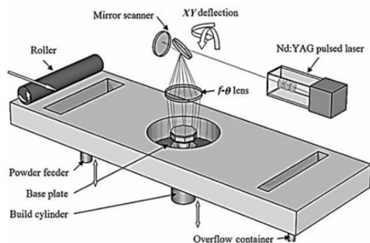
Fig. 2 SLS system configuration [9]
