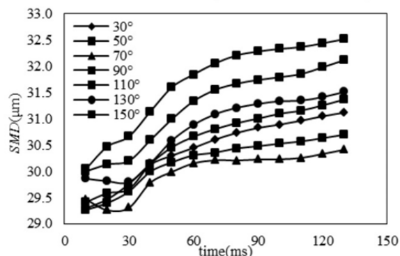
Fig. 10 The SMD of the droplets based on the longitudinal angle of the two injectors ( x_1=x_2=30\text{mm} , \varphi=180^\circ , \alpha=15^\circ )
