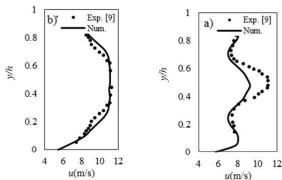
Fig. 2 velocity profile in the present study and the experimental results [9] in \theta_1 = \theta_2 = 60^\circ (a) and \theta_1 = \theta_2 = 120^\circ (b) ( x_1 = x_2 = 30\text{mm} , \varphi = 180^\circ , \alpha = 80^\circ )
