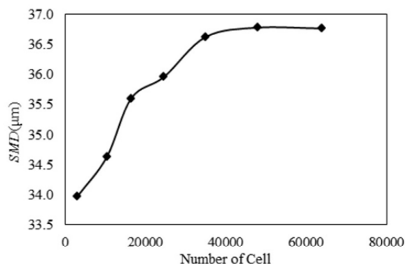
Fig. 4 The effect of the number of cells on the SMD
