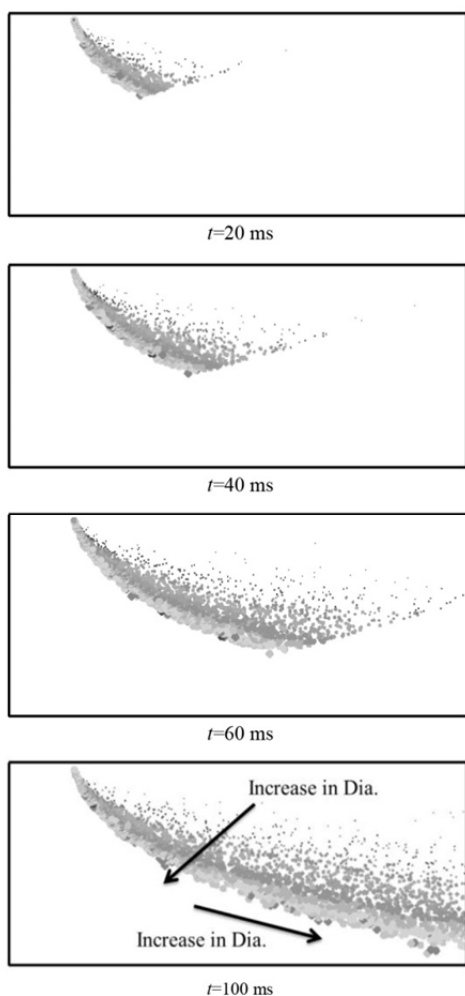
Fig. 5 The spray injected in an air flow ( \theta_1 = 70^\circ , x_1 = 30\text{mm} , \alpha = 15^\circ )
