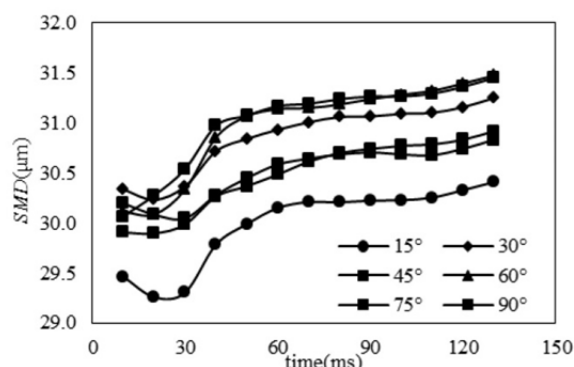
Fig. 9 The SMD of the droplets based on the time in various cone angles ( x_1=x_2=30\text{mm} , \theta_1=\theta_2=70^\circ , \varphi=180^\circ )
