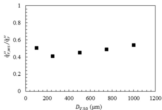
Fig. 10 The profile of the ratio of radiative flux after activating the sprinklers to the radiative flux before activating them with the median droplet diameter in the upstream area
