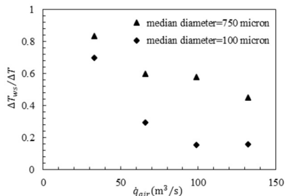
Fig. 13 The profile of the ratio of temperature difference after activating sprinklers to the temperature difference before activating them with the air flow rate
