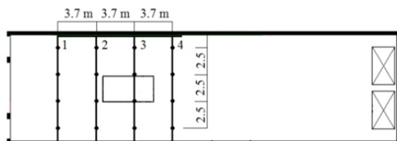
Fig. 16 The location of the sprinklers in the tunnel
