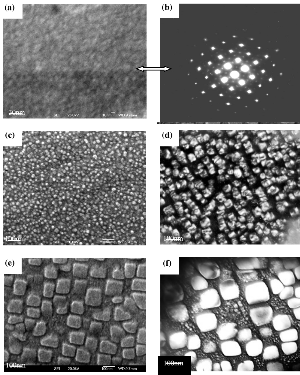
Fig. 1. FEGSEM (left hand) and dark field TEM (right hand) micrographs of solutioned and quenched samples; (a) Ni-11.56at%Al; (b) Selected area electron diffraction pattern of Ni-11.6 at.%Al alloy. The foil was oriented in \langle 001 \rangle direction and the superlattice reflections (weak points) are \{100\} and \{110\} type. (c,d) Ni-15.3 at.%Al; (e,f) Ni-17.5 at.%Al.
