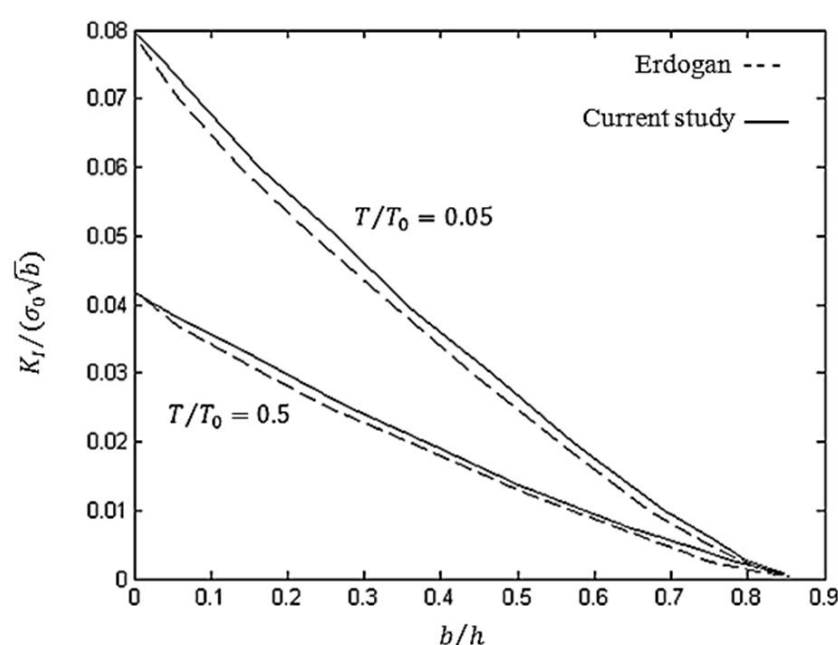
Fig 12. Nondimensional Stress intensity factor foe edge crack with \omega = \ln(2) , \beta = \ln(5)
