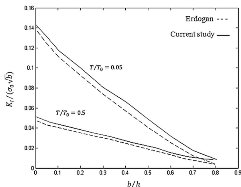
Fig 13. Nondimensional Stress intensity factor foe edge crack with \omega = \ln(2) , \beta = \ln(10)
