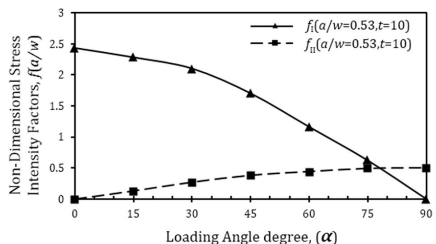
Fig. 14 Non-dimensional stress intensity factors vs. loading angle, t (mm)
