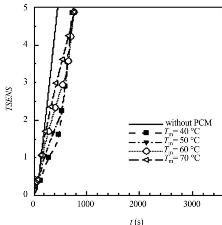
Fig. 9 Time variations of thermal sensation index under scorching conditions by using protective clothing with arrangement of Case 2
