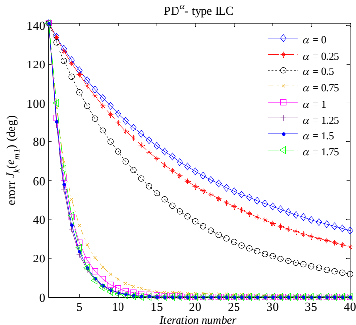
Fig. 11 Maximum absolute angular tracking errors versus the iteration number, Comparison of PD α -type ILC with different \alpha and k = 1, \dots, 40 .
