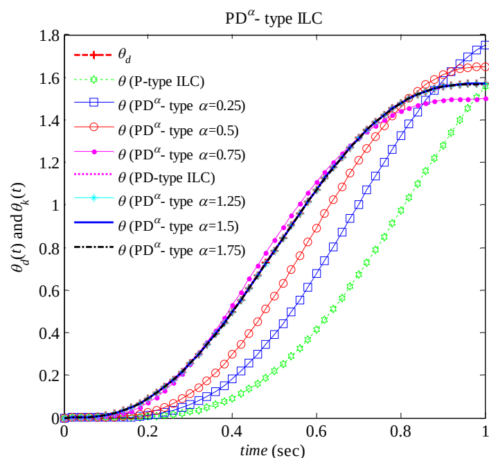
Fig. 12 Desired and the output diagram by using updating law PD α -type ILC for different values of \alpha and k=40 .
