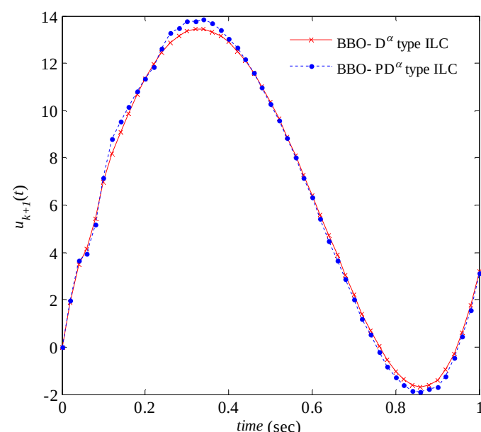
Fig. 16 The control signal for different values of \alpha , by using updating laws BBO- D^\alpha -type ILC and BBO- PD^\alpha -type ILC for k=10 .
