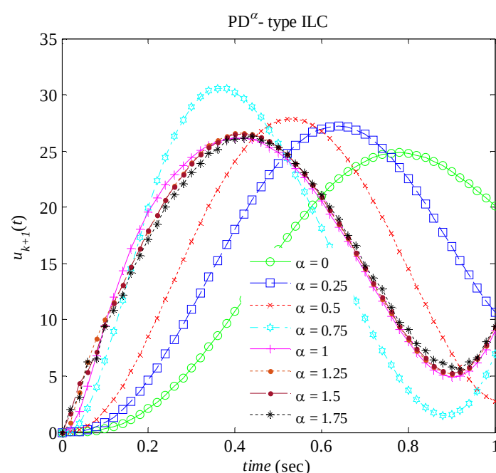
Fig. 13 The control effort for different values of \alpha , by using updating law PD^\alpha -type ILC and k=40 .
