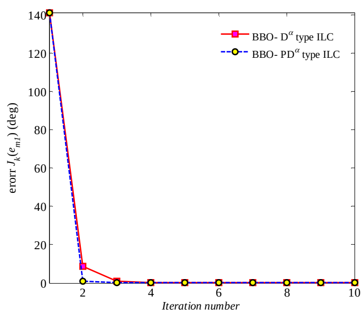
Fig. 15 Maximum absolute angular tracking errors versus the iteration number, for D^\alpha -type ILC and PD^\alpha -type ILC using the BBO algorithm.
