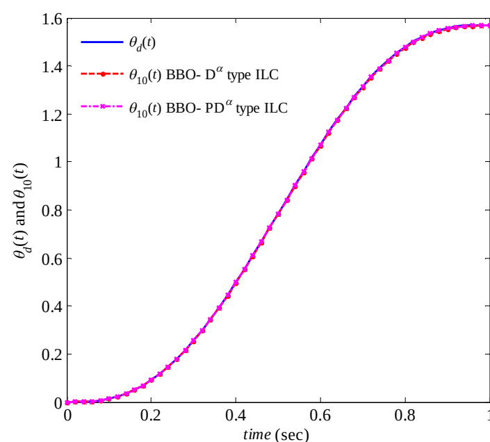
Fig. 17 Desired and the output trajectory of the robot arm of BBO- D^\alpha -type ILC and BBO- PD^\alpha -type ILC updating laws, for k=10 and different values of \alpha .
