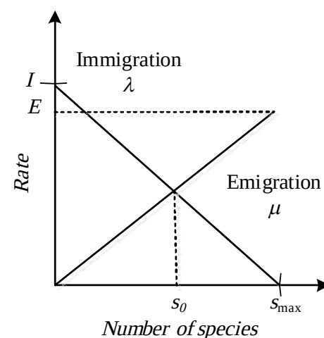
Fig. 3 Species model of a single habitat
