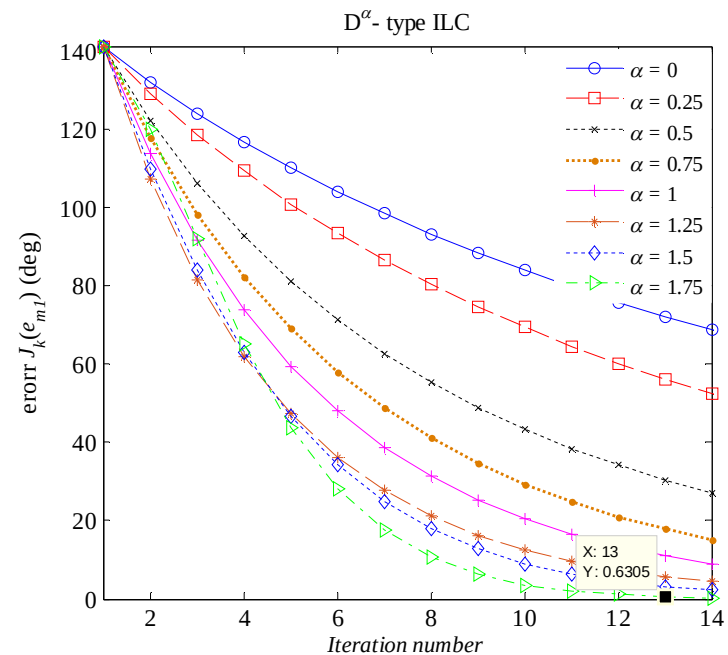
Fig. 9 Maximum absolute angular tracking errors J_k(e_{m1}) , versus the iteration number, Comparison of D α -type ILC with different \alpha . With respect to the iteration number 14.
