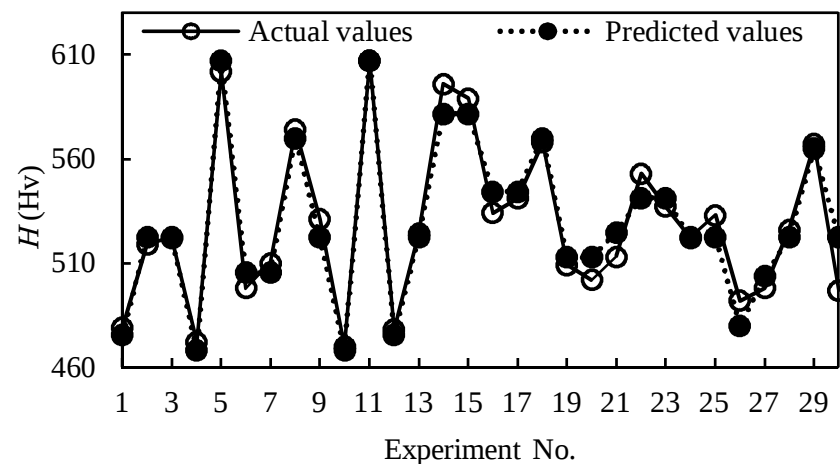
Fig. 5 Comparison of predicted and empirical results for microhardness in each experiments
