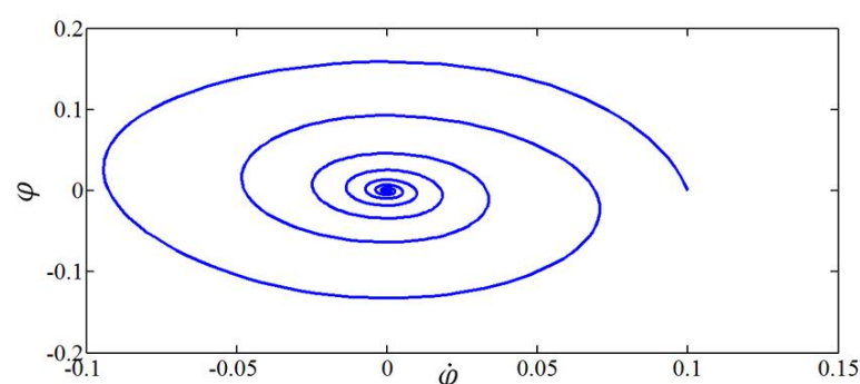
Fig. 4 Phase diagram of the harmonically excited roll motion
