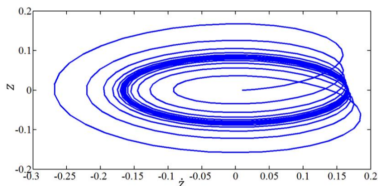
Fig. 6 Phase diagram of the harmonically excited heave motion
