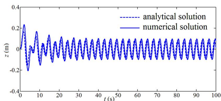
Fig. 5 Comparison of the analytical and numerical heave motion
