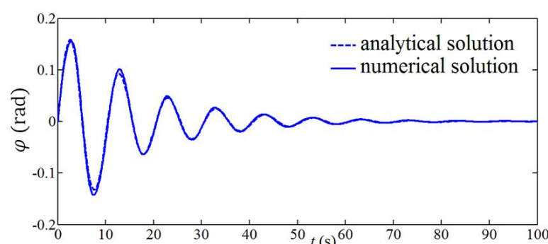
Fig. 3 Comparison of the analytical and numerical roll motion
