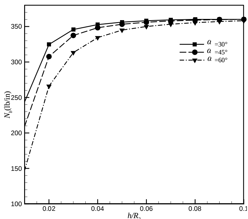
Fig. 10 Effect of h/R_2 on the buckling load in differential quadrature method
