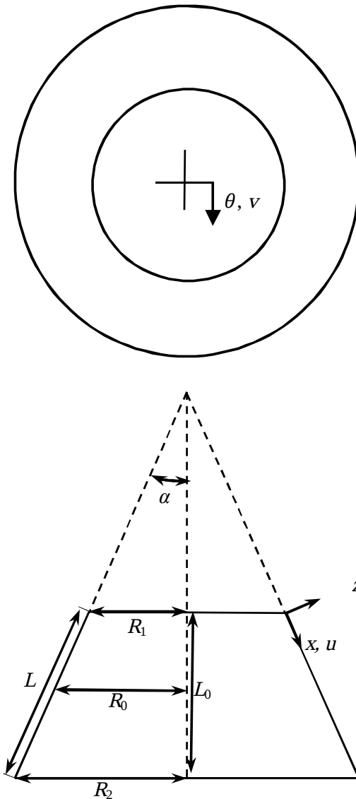
Fig. 1 Conical shell coordinate system
