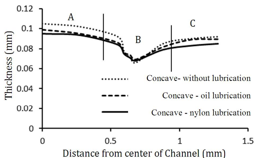
Fig. 24 Comparing the concave sample thickness distribution in longitudinal direction in three cases, i.e. without lubricant, oil lubricant and nylon lubricant
