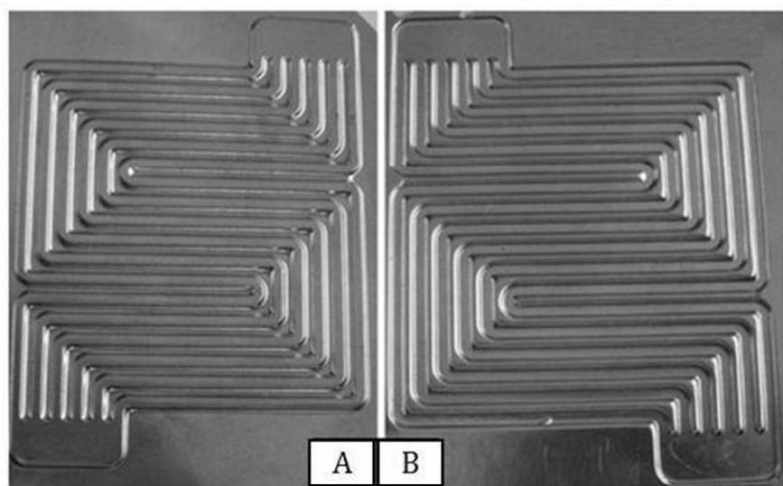
Fig. 26 Sample of a metal bipolar plate fabricated by rubber pad forming with nylon lubricant and convex die: (a) front view of the bipolar plate and (b) back view of the bipolar plate
