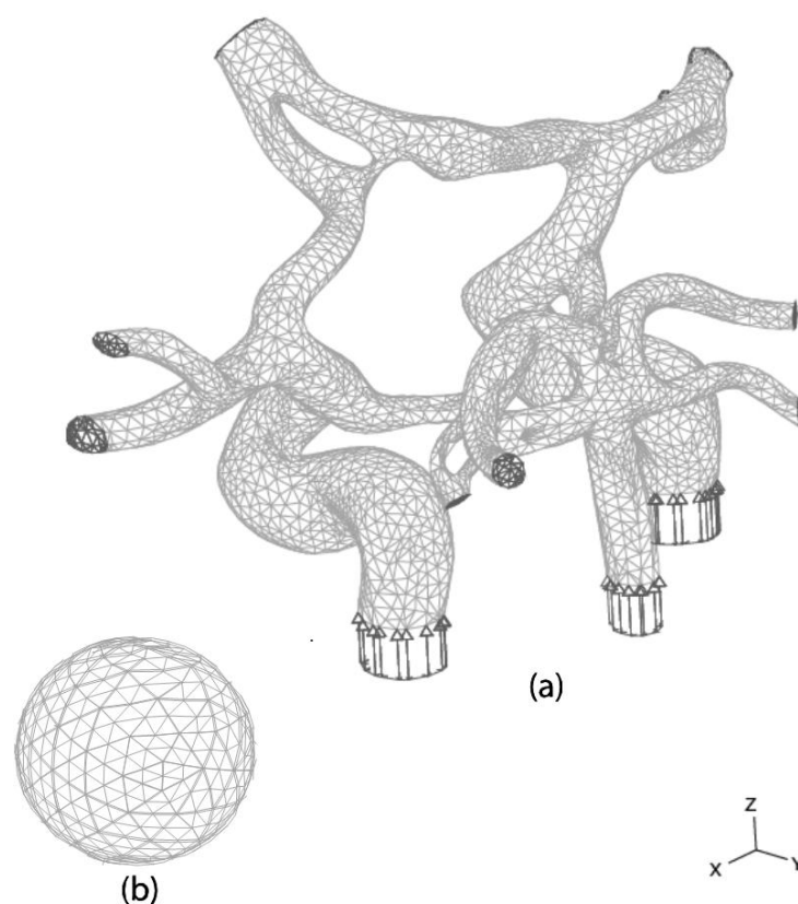
Fig. 3 Discretized model for (a) fluid and (b) solid domain
