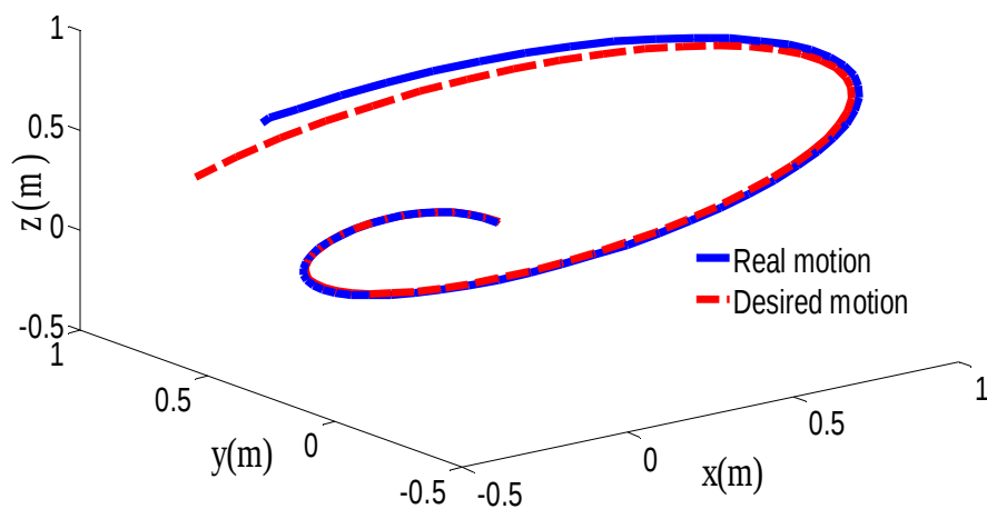
Fig. 12 Three-dimensional movement of the movable plate
