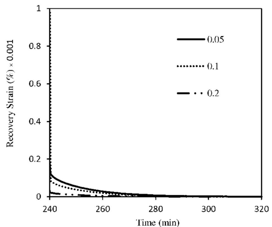
Fig. 11 Effects of effective interphase thickness on the recovery strain of the glass/epoxy composite under axial loading, applied stress equals to 30 MPa
