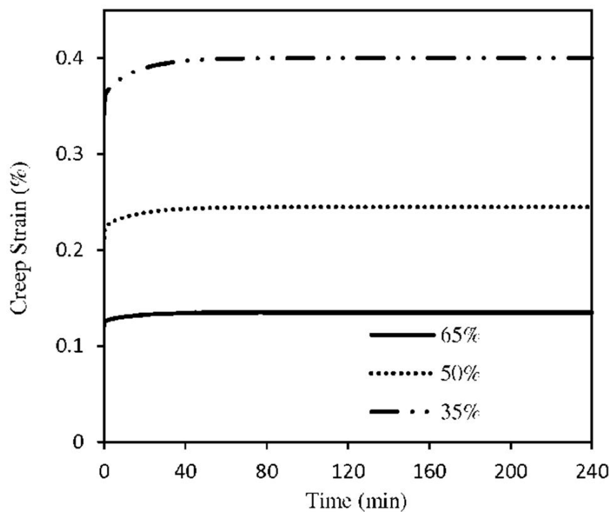
Fig. 16 Effects of fiber volume fraction on the creep strain of the glass/epoxy composite under transverse loading, applied stress equals to 30 MPa
