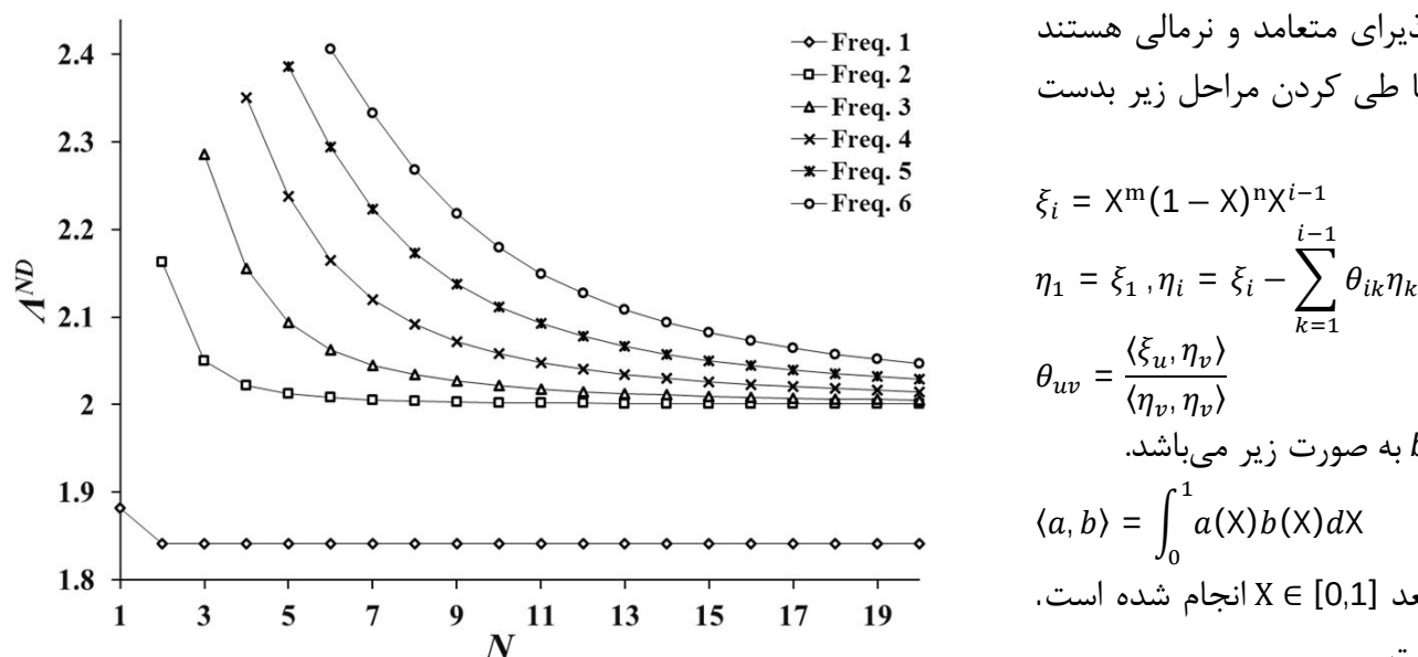
Fig. 2 Convergence of first six frequency parameters for a C-C1 nanorod
