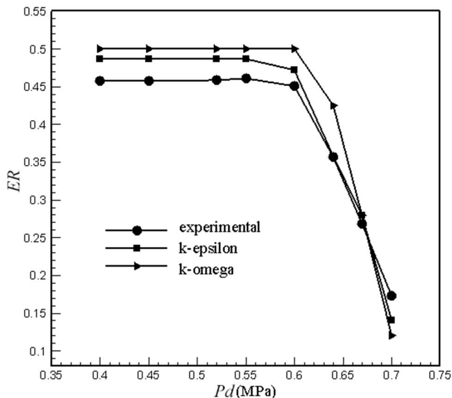
Fig. 1 Entrainment ratio variations with discharged pressure in two different turbulence models
