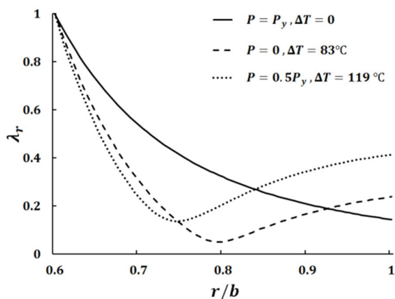
Fig. 9 Yield variable changes throughout thickness in yield onset of material with 3 d row properties in Table 3
