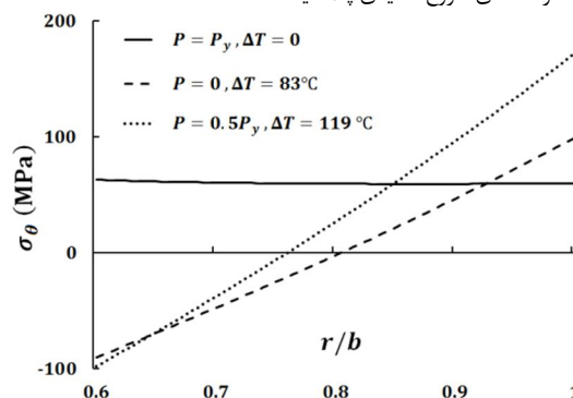
Fig. 8 Tangential stresses changes throughout thickness in yield onset of material with 3 d row properties in Table
