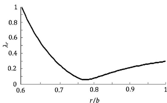
Fig. 10 Yield variable curve throughout thickness for a=0.06 m, b=0.1 m, m_1=3 , m_2=-1.1 , m_3=3 , m_4=2 and \Delta T=157^{\circ}\text{C}
