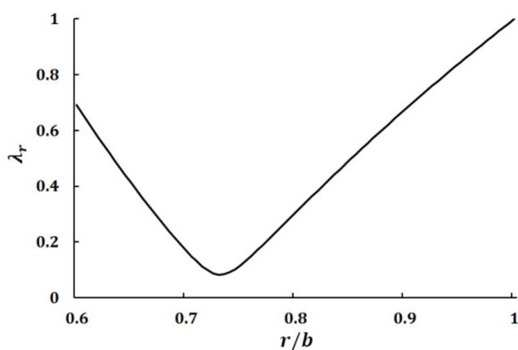
Fig. 11 Yield variable curve throughout thickness for a=0.06 m, b=0.1 m, m_1=2 , m_2=-1.5 , m_3=-1.5 , m_4=-3 and \Delta T=328^{\circ}\text{C}
