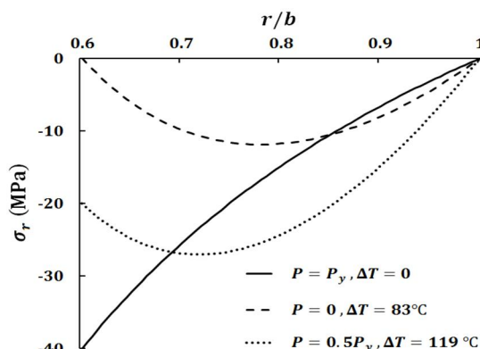
Fig. 7 Radial stresses changes throughout thickness in yield onset of material with 3 d row properties in Table
