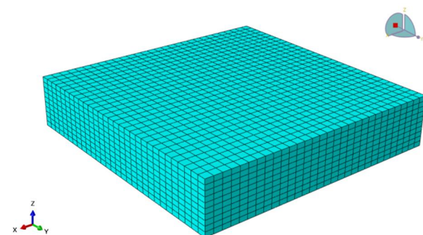
Fig. 3 The plate modeled in ABAQUS software with the meshes used for numerical analysis
