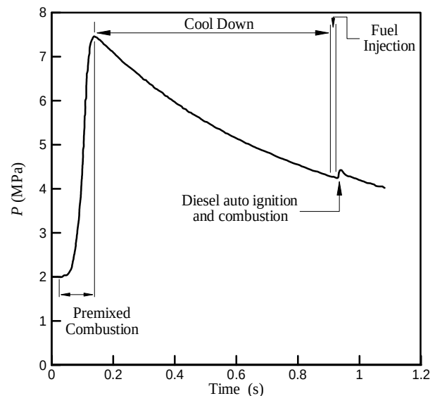
Fig. 2 Simulation to product core ambient of 1000 K, density 14.8 kg/m³, 21% O₂ at the time of diesel fuel injection [8]
