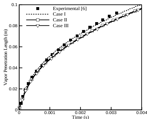
Fig. 14 Predicted vapor penetration length for three considered droplet diameter distribution
