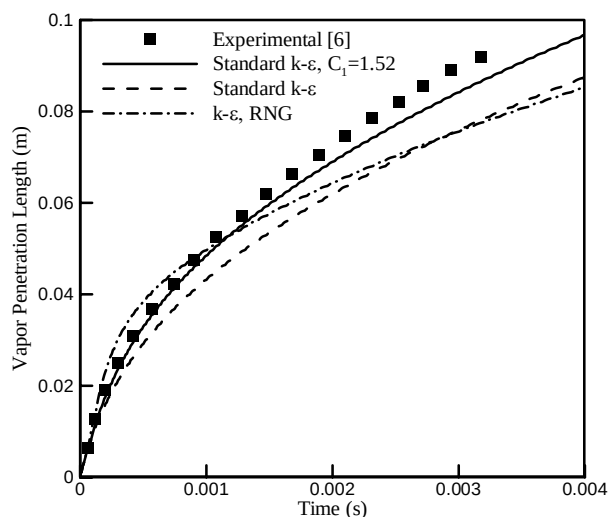
Fig. 8 Effect of turbulence model on spray characteristics
