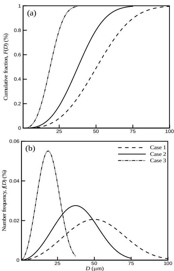
Fig. 10 Considered droplet diameter distribution: (a) Cumulative number distribution and (b) Number frequency distribution
