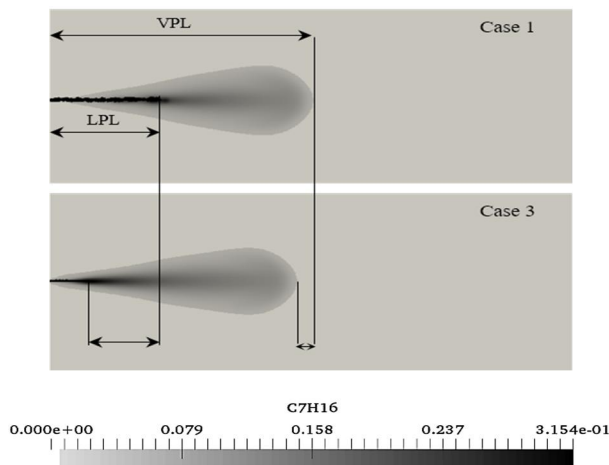
Fig. 15 Compare of liquid and vapor penetration length for case 1 and 3 after 113 ms after injection
