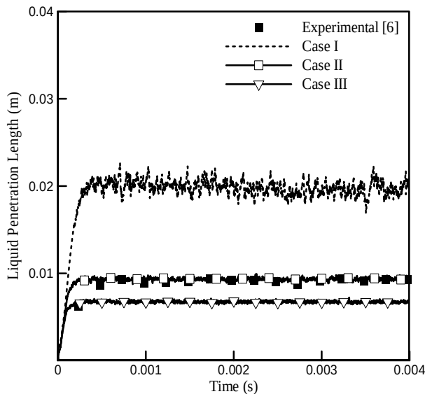
Fig. 12 Predicted liquid penetration length for three considered droplet diameter distribution
