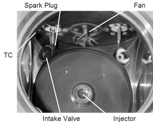
Fig. 1 Experimental sample of case study [7]
