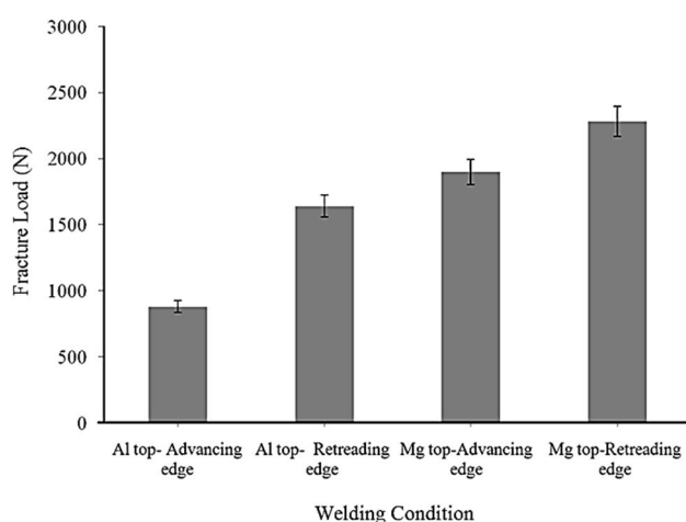
Fig. 12 Results of shear tensile tests of Al/Mg joints
