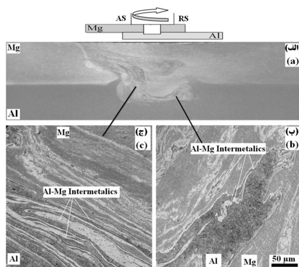
Figure 5 Microstructure of different zone from interface in Mg top-Retreading edge joints
