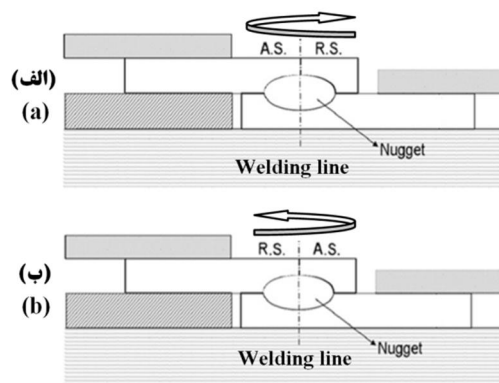
Fig. 3 Different configuration of welding according to tool rotation direction (a) Retreading edge (b) Advancing edge
