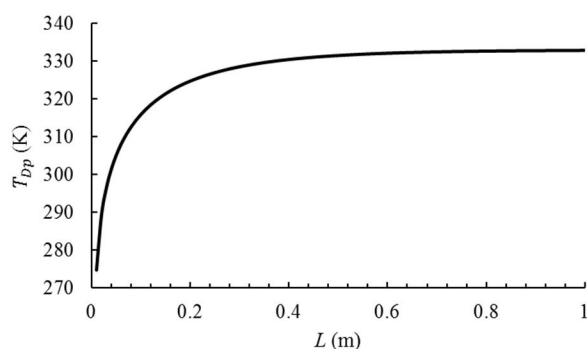
Fig. 5 Graph of dew point variations along the length of channel
