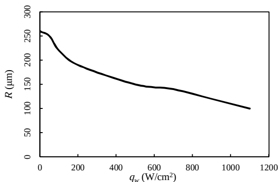
Fig.11 Kovalev critical radius vs. wall heat flux
