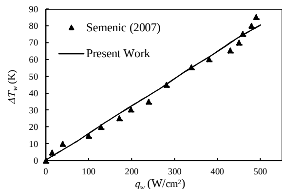
Fig.8 Comparison between Numerical results and Semenik [20] data for the wick with characteristics shown in Fig.6
