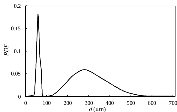
Fig.7 Probability mass function for one of Semenik's biporous wicks [18]
