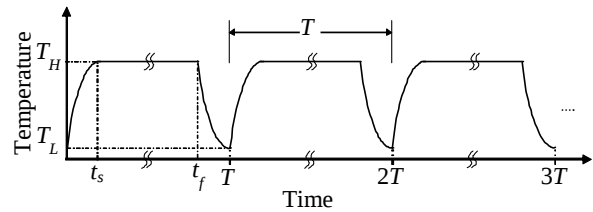
Fig. 12 Schematic figure of applied thermal cycles on the top and bottom walls of model
