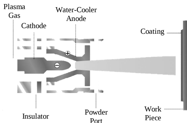
Fig. 3 Schematic figure of air plasma spraying process
