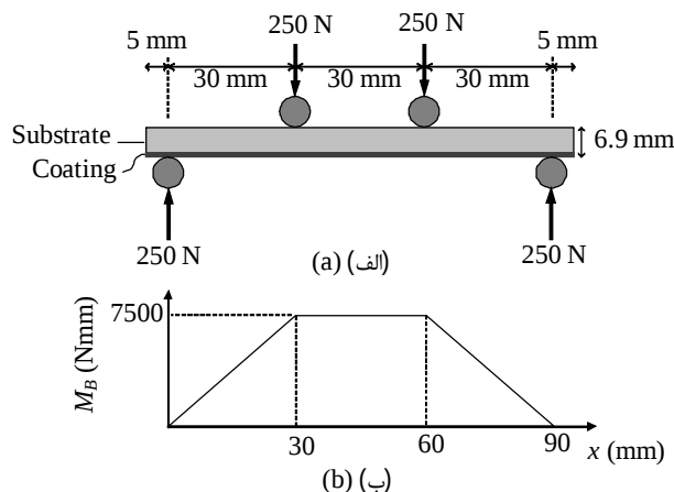
Fig. 5 (a) Geometry of 4-point mechanical bending load, (b) Bending moment of applied load along the length of specimen
