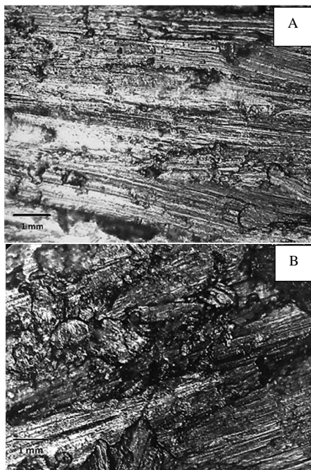
Fig. 10 Optical microscope images of electro discharge machined surfaces. A: sample machined with 8A pulse current and 25μs pulse time. B: sample machined with 32A pulse current and 400μs pulse time.
