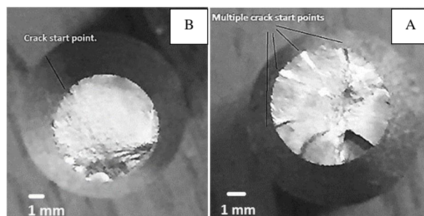
Fig. 9 Cross-section of samples after fatigue. A. Sample with maximum roughness. B. Sample with minimum roughness
