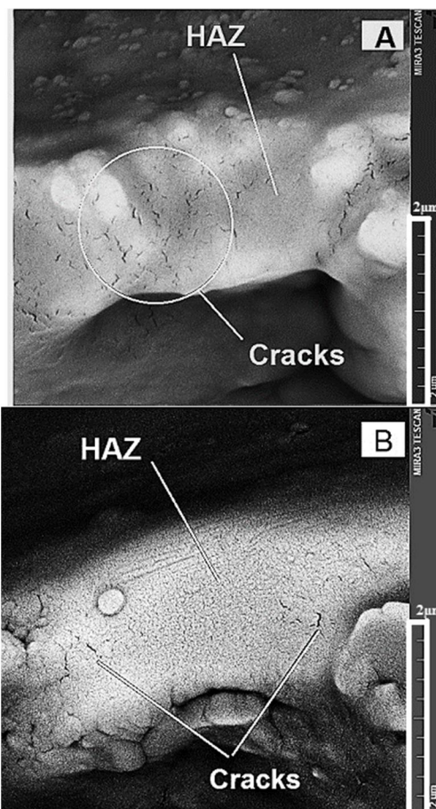
Fig. 5 SEM images showing HAZ region of samples. A. pulse current 32A and pulse time 400μs. B. pulse current 8A and pulse time 100μs
