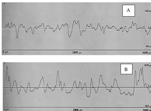
Fig. 8 Roughness profile of samples. A. sample machined with 8A pulse current and 25μs pulse time. B. sample machined with 32A pulse current and 100μs pulse time.
