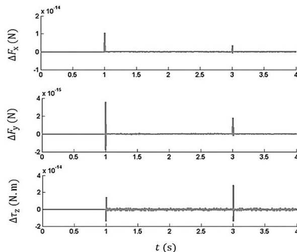
Fig. 7 Difference of obtained forces and moments from virtual and dynamic model of robot.
