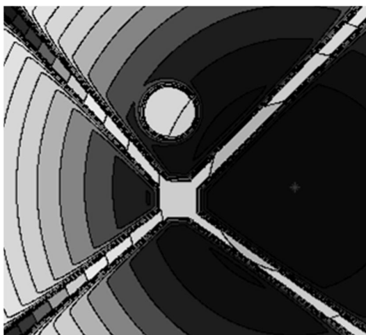
Fig. 12 Potential field of goal, obstacle, cables and dynamic plane
