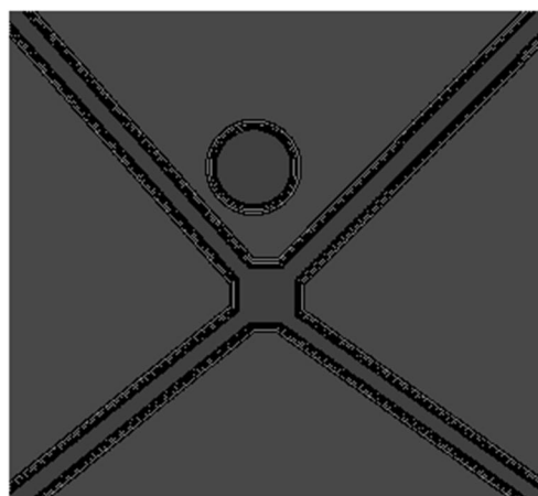
Fig. 10 Potential field of obstacle and cables and dynamic plane
