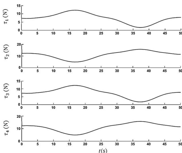
Fig. 20 Cables forces in trajectory of the obtained path for Fig. 18
