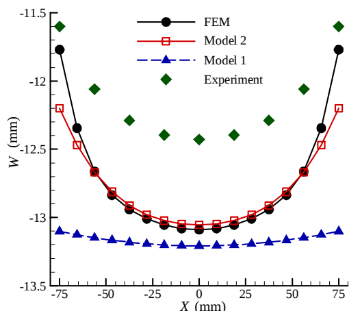
Fig.11 Out of plane displacement of the path L_2 at 25°C
