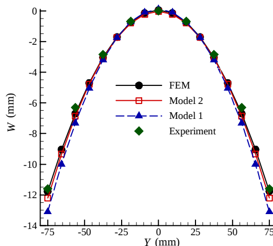
Fig.10 Out of plane displacement of the path L_1 at 25°C
