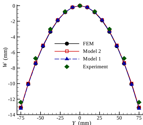
Fig.12 Out of plane displacement of the path L_3 at 25°C
