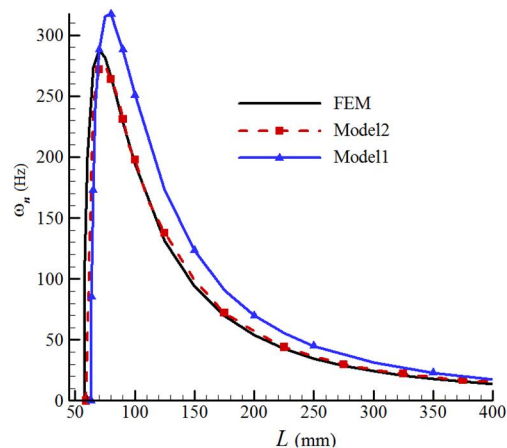
Fig.16 First natural frequency of the square laminate versus side length at 25 °C
