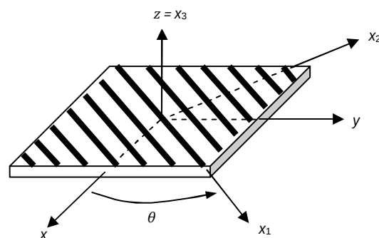
Fig.a-1 Schematic of a lamina in global and local coordinate systems
