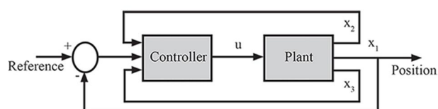
Fig. 7 Schematic block diagram of the close-loop system
