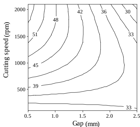
Fig. 23 Interaction effect of cutting speed and gap
