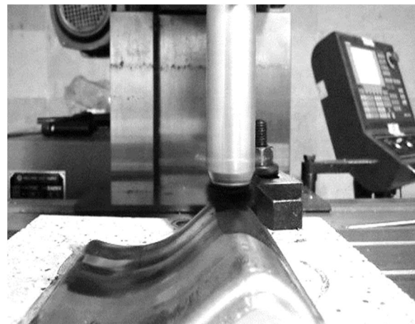
Fig. 17 Performing MAF process
