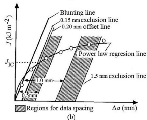
Fig. 6 J-R curve and J_{IC} data-qualifying schemes according to ASTM standards; a: E813-81 و b: E813-87 [24,25]
