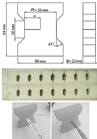
Fig. 12 Fracture butterfly-shape specimens and their preparing
