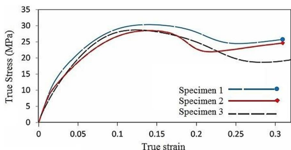
Fig. 10 True strain-stress curves obtained from tension tests
