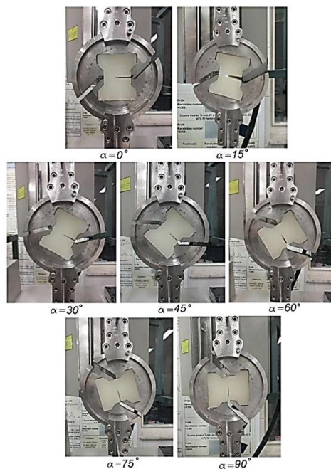
Fig. 13 Fracture tests under mode-I, mode-II and I/II mixed-mode states with increment of 15 degrees for loading angle
