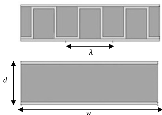
Fig. 1 A schematic cross section of two specimen; simple and square corrugated core.
