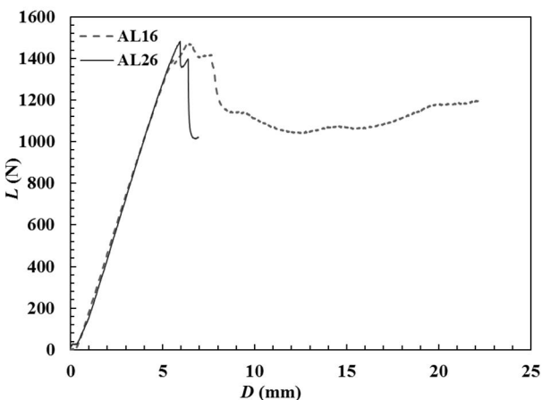
Fig. 15 force-displacement plots for AL16, AL26
