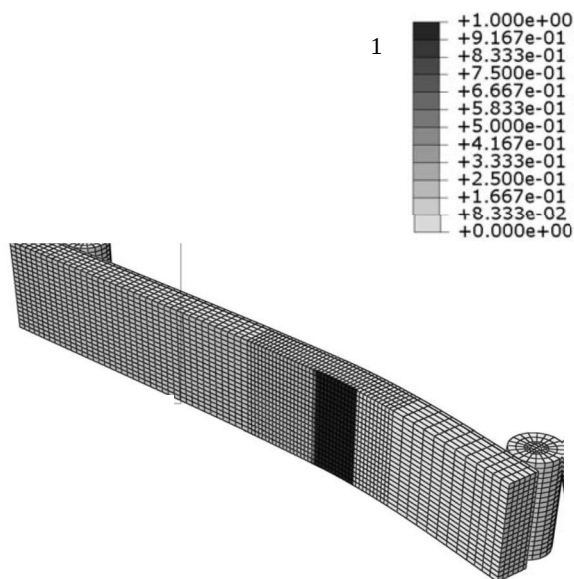
Fig.18 comparison of numerical and experimental result for simple core
