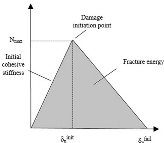
Fig. 8 bilinear traction-separation
