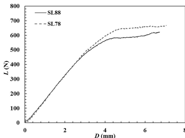
Fig. 13 force-displacement plots for SL78, SL88
