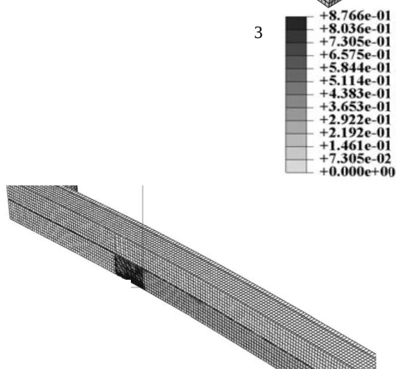
Fig. 20 damage scalar parameters 1) simple core, 2) 8 layer skin and square core, 3) 6 layer skin and square core
