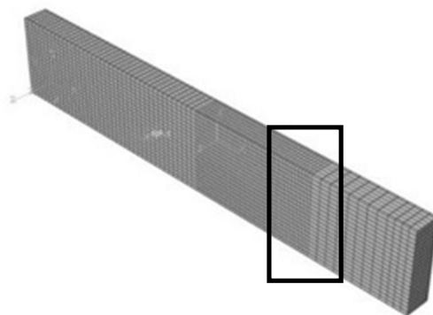
Fig. 10 increasing the mesh density in the crack tip
