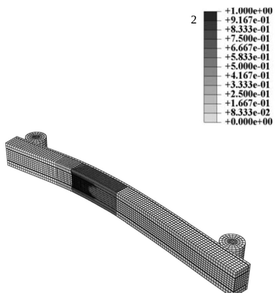
Fig. 19 comparison of numerical and experimental result for square corrugated core
