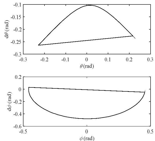
Fig. 10 Limit cycle of the elastic biped at the period-one gait for the slope of \gamma for the swing and stance leg are plotted. Biped walked 1000 cycles without falling over.
