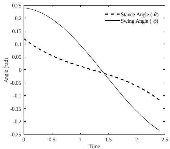
Fig. 2 A typical step of elastic biped at the slope of \gamma
