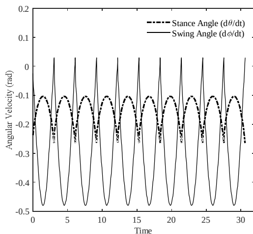
Fig. 9 Changes of the biped angular velocities through period-one gait at the slope of \gamma
