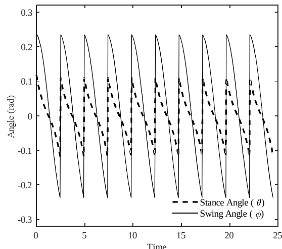
Fig 5 Period-one gait for the elastic biped robot at the slope of \gamma . Biped's angles are not affected by the vibrations of the stance leg.
