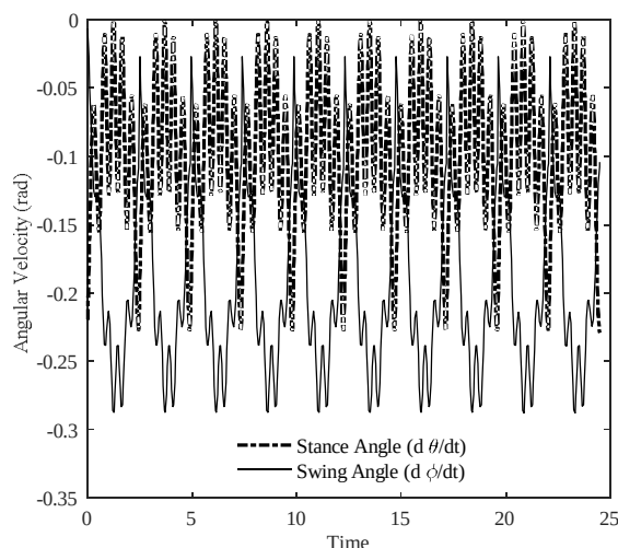
Fig. 6 Time evolution of angular velocities of the elastic biped at the slope of \gamma through period-one gait. Despite oscillations of the stance leg, he biped walks smoothly.
