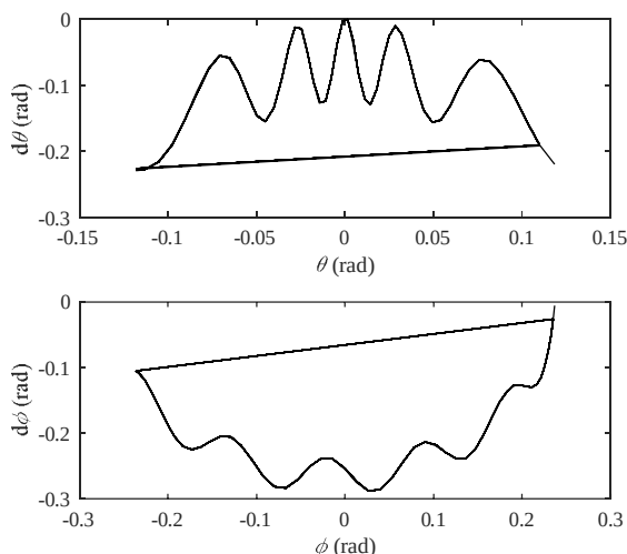
Fig. 7 Phase plane diagram of the elastic biped at period-one gait for the slope of \gamma
