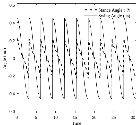
Fig. 8 Period-one gait for the elastic biped at the slope of \gamma
