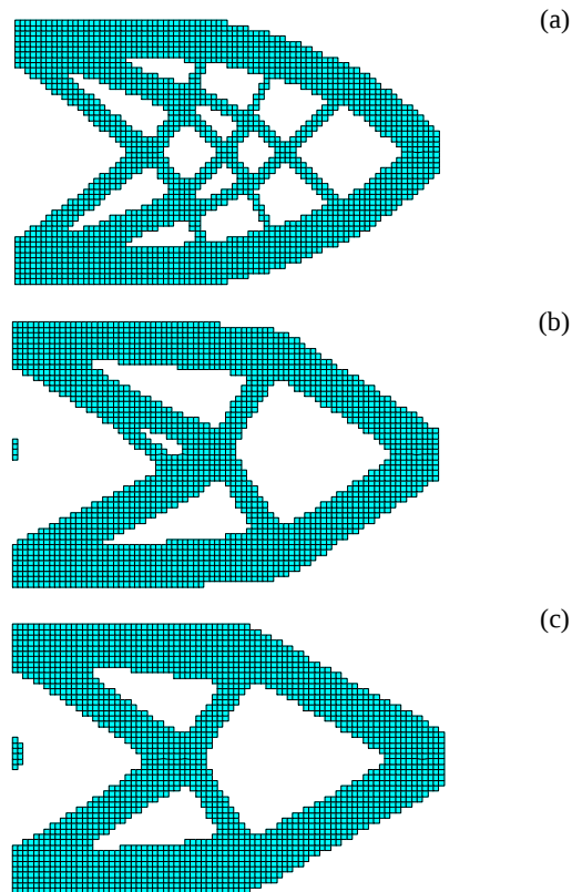
Fig.5 Optimal topology for cantilever beam with ER = 2\% : (a)
