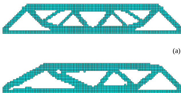
Fig.9 Optimal topology for beam with ER = 1%:
