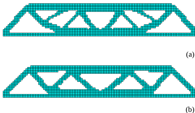
Fig.8 Optimal topology for beam with ER = 2%:
