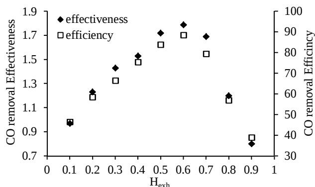
Fig. 15 Effect of exhaust height on CO removal efficiency and effectiveness
