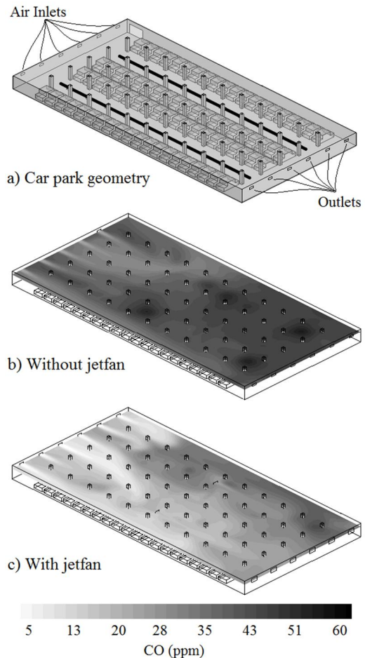
Fig. 16 CO distribution in car park, h=2 m, t=60 min
