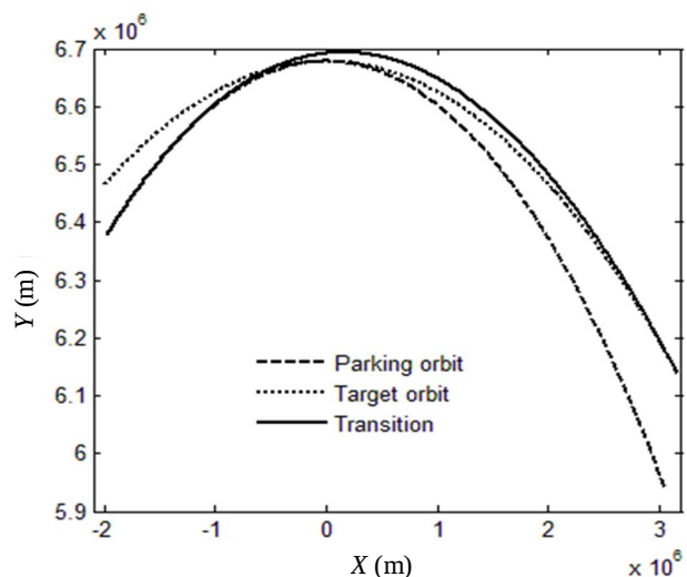
Fig. 12 Flight path in the first phase of transition
