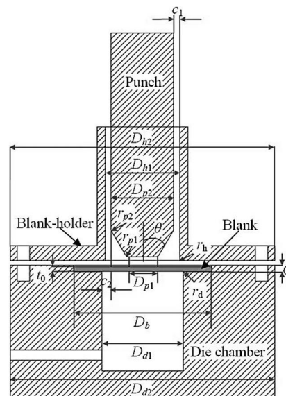
Fig. 2 Representation of parametric dimensions of hydroforming die set used in this research
