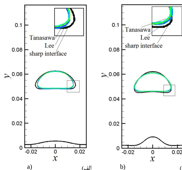
Fig. 5 Detached bubbles from the vapor film in three phase change models, a) The first detached bubble, b) Detached bubble in semi steady state period
