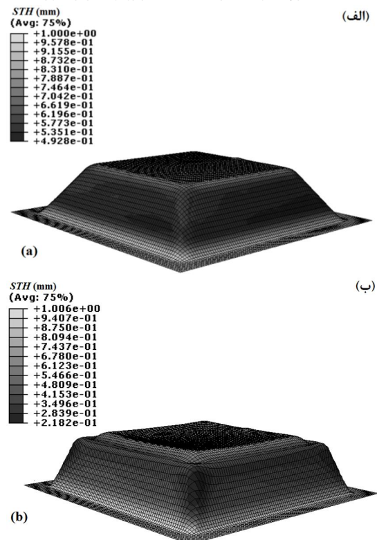
Fig.17 The predicted thickness distribution of the first strategy: a) the first stage b) the second stage
