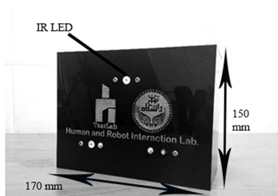
Fig. 2 Isometric view of the solid object and IR LEDs
