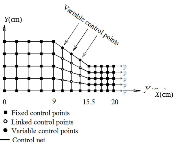
Fig. 15 Design variables for two-dimensional fillet example
