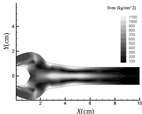
Fig.13 Optimum design and final stress contour plot
