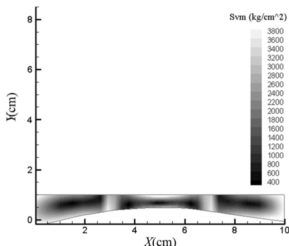
Fig. 21 von Mises stress Cantours with optimum shape
