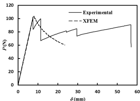
Fig. 17 Load – displacement curve with crack length 60 m
