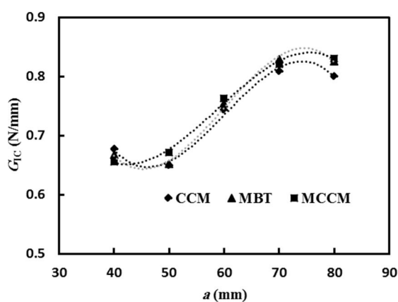
Fig. 11 Experimental R-curves obtained by the MBT, CCM &amp; MCCM
