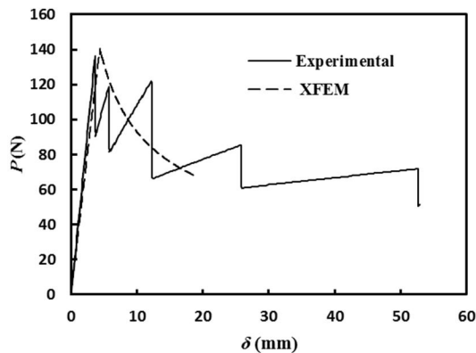
Fig. 15 Load – displacement curve with crack length 40 mm
