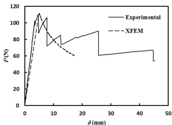
Fig. 16 Load – displacement curve with crack length 50 mm
