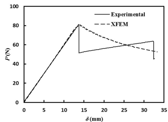
Fig. 19 Load - displacement curve with crack length 80 mm
