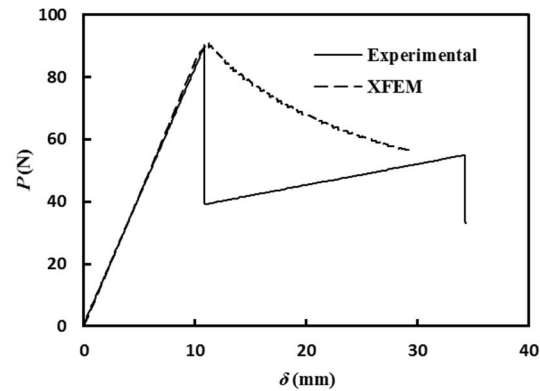
Fig. 18 Load - displacement curve with crack length 70 mm
