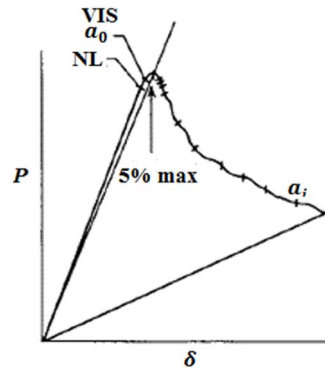
Fig. 4 Crack growth initiation criteria [17]
