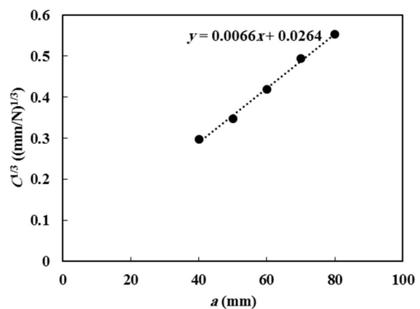
Fig. 8 C^{1/3} vs. crack length for DCB specimens
