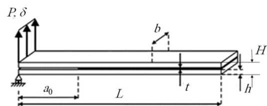
Fig. 1 Schematic representation of the DCB specimen [4]
