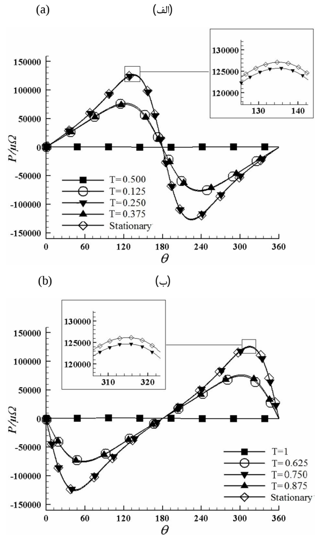
Fig. 5 Dimensionless pressure profile ( R_f = 0.001 & \varepsilon = 0.54 ),
