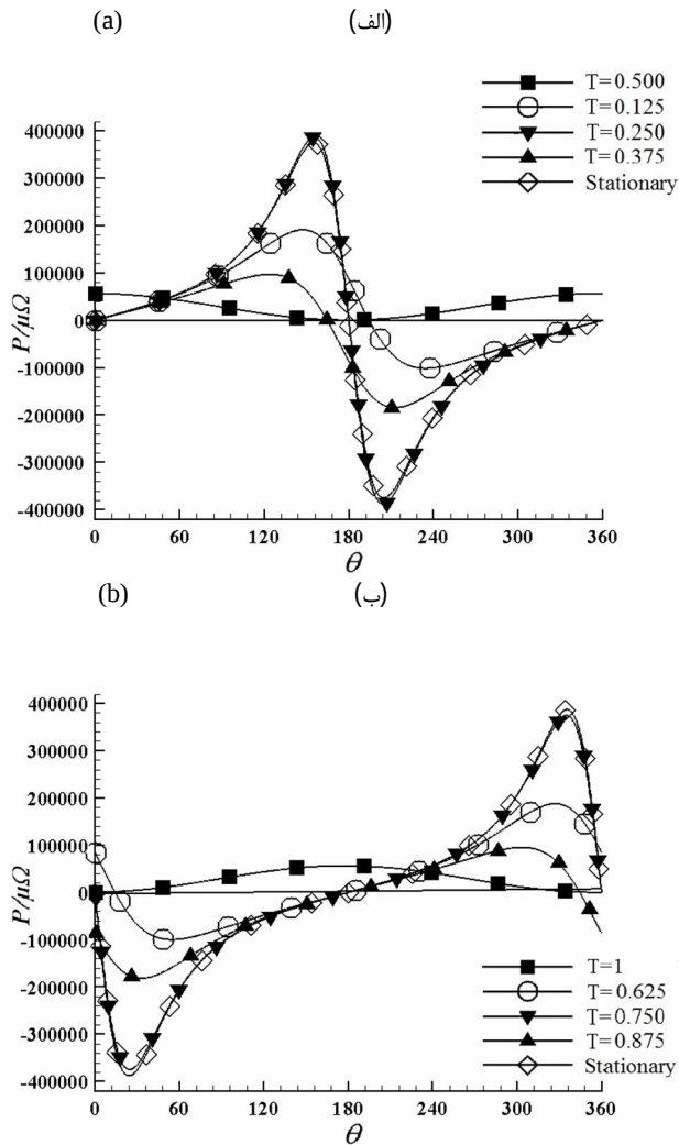
Fig. 8 Dimensionless pressure profile ( R_f = 0.1 & \varepsilon = 0.8 ),
