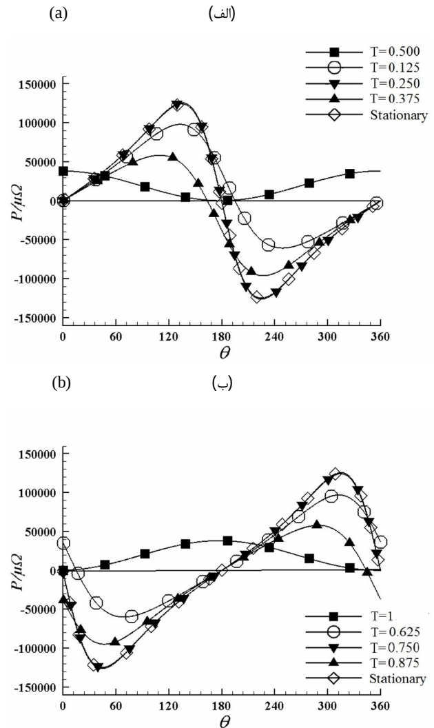
Fig. 7 Dimensionless pressure profile ( R_f = 0.1 & \varepsilon = 0.54 ),
