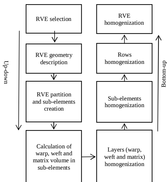
Fig. 1 Diagram of steps of micromechanical model
