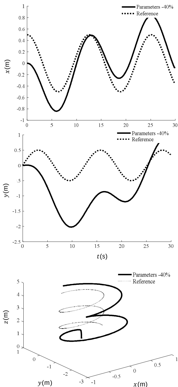
Fig. 3 Position of (X,Z) and path tracking with increasing uncertainty in mass 40% and without identification
