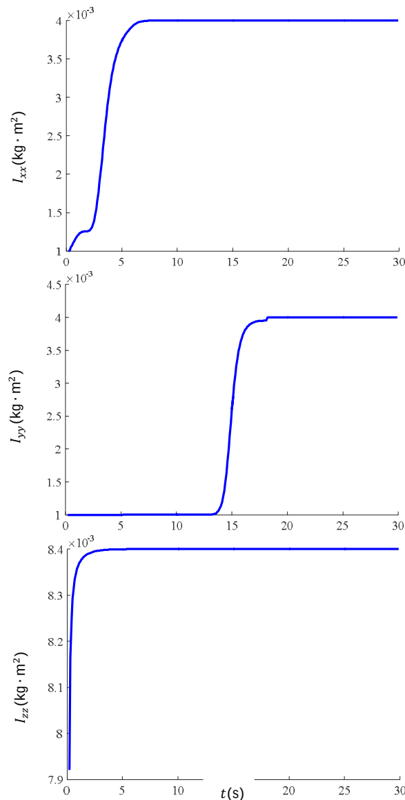
Fig. 9 Estimation of inertia matrix ( I_{xx}, I_{yy}, I_{zz} ) parameters with recursive least square
