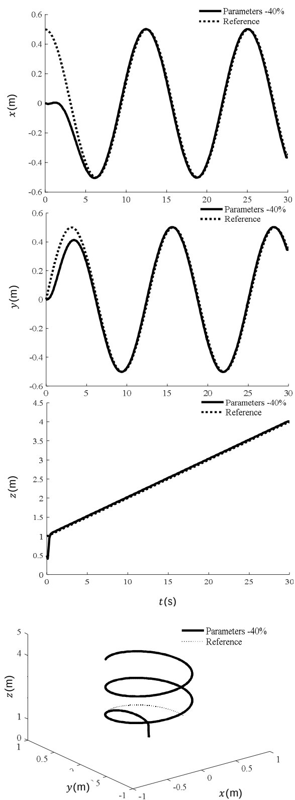
Fig. 6 Position ( X, Y, Z ) and path tracking with external disturbances and uncertainty with RLS
